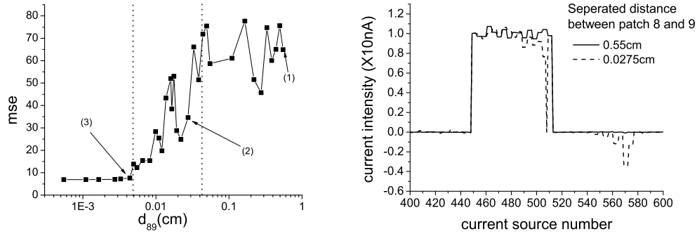
FIGURE 3. A (left panel): mse value vs. the separation d_{89} between patches 8 and 9. The distances d_{89}=0.55 , 0.0275 and 0.0035 cm are marked out and labeled (1), (2) and (3), respectively. B (right panel): Reconstructed \langle \mathbf{r} \rangle vs. source number for the cases (1) (solid line) and case (2) (dashed line) in A.
